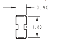
Antenna Pad Layout
