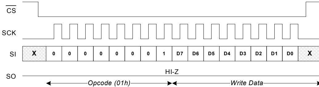
Figure 66. WRSR Instruction in DPI Mode
