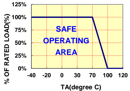
DERATING CURVE
