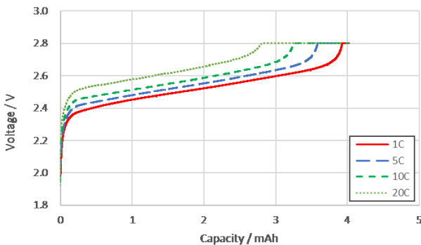
Charge characteristics
