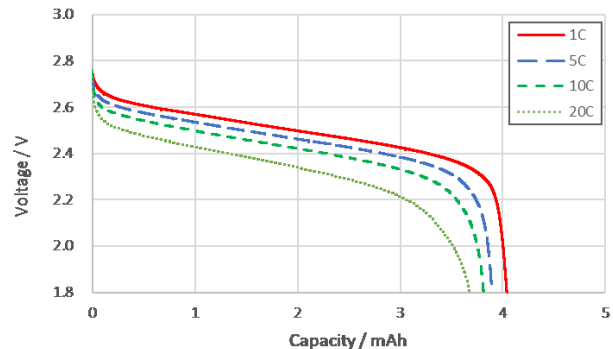
Discharge characteristics
