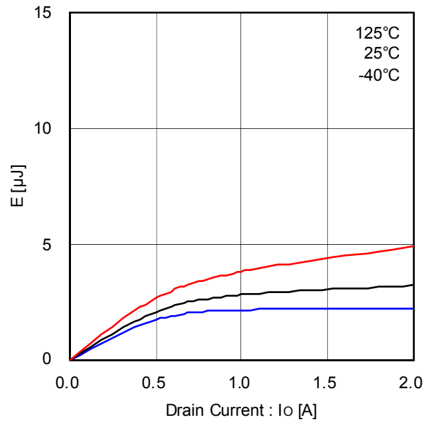
Figure 24. High Side Recovery Loss (VDC=150V)
