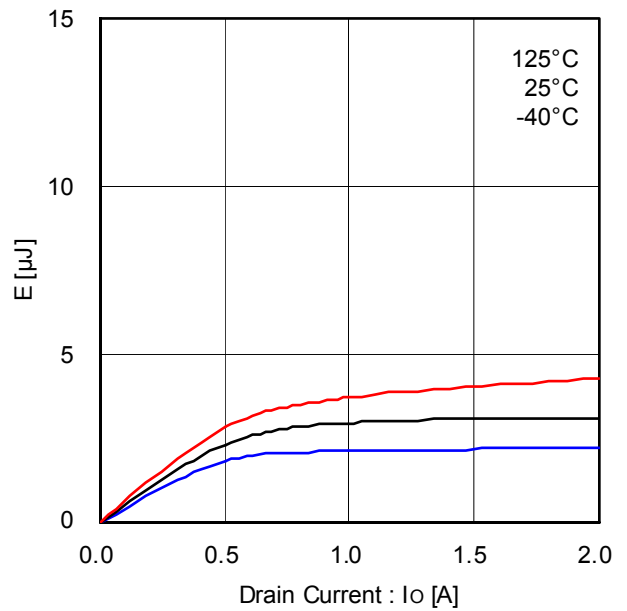
Figure 26. Low Side Recovery Loss (VDC=150V)
