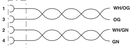
Contact assignment of the M12 socket
