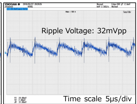
V_{IN}=100Vac , I_{OUT}=167mA
