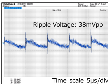
V_{IN}=230Vac , I_{OUT}=100mA
