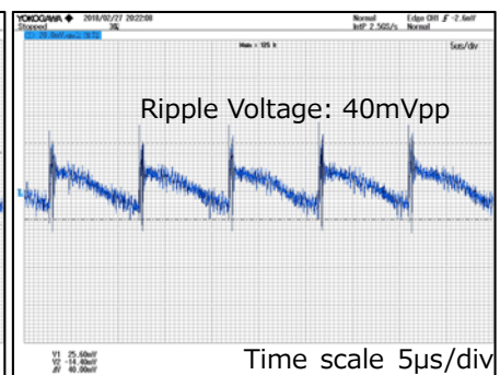
V_{IN}=230Vac , I_{OUT}=167mA
