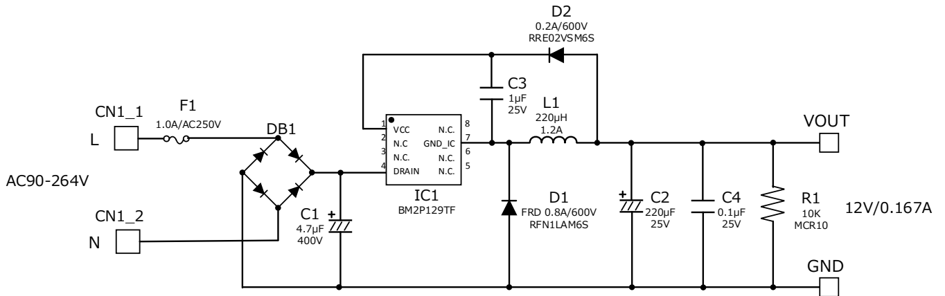
Figure 3. BM2P129TF-EVK-001 Schematics
