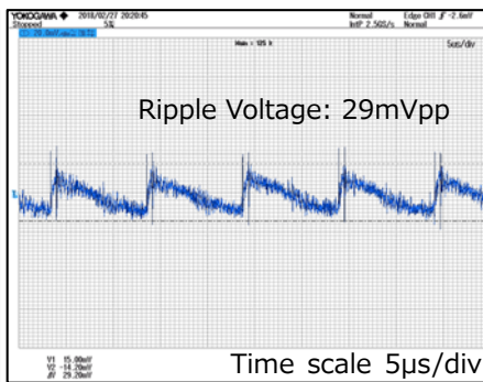
V_{IN}=100Vac , I_{OUT}=100mA
