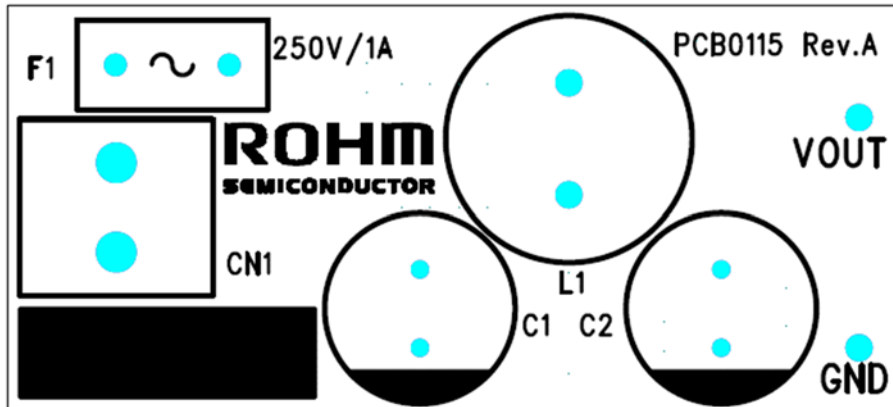
Figure 4. Top Silkscreen (Top view)
