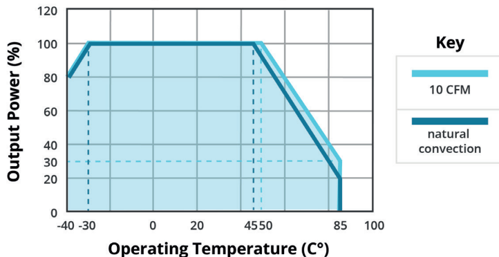
TEMPERATURE DERATING CURVE (-CNF versions)
