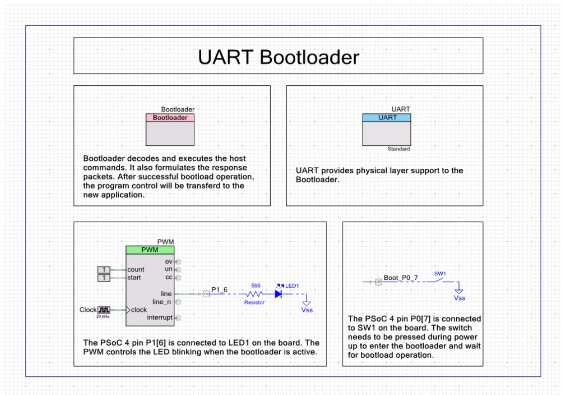
Figure 5-1. UART Bootloader
