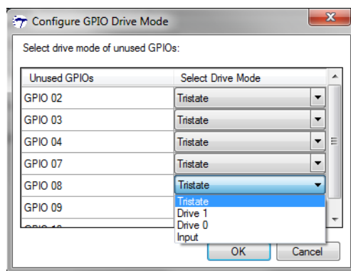
Figure 6-12. Configuring GPIO Drive Mode
