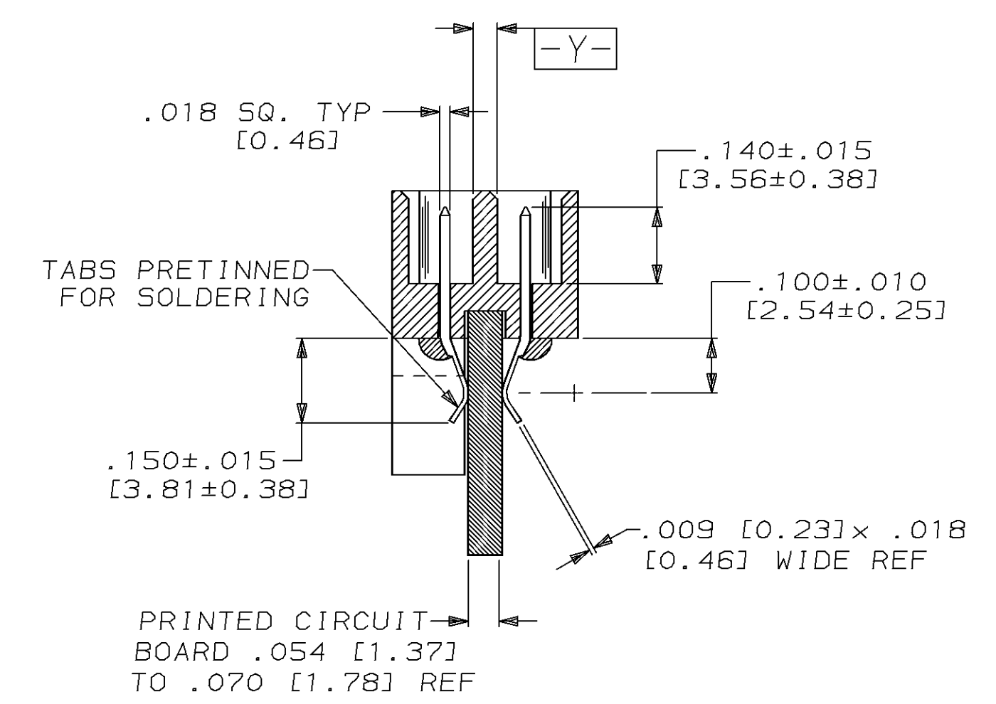
SECTION T-T
