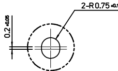
DETAIL 1 (SCALE 5:1)
