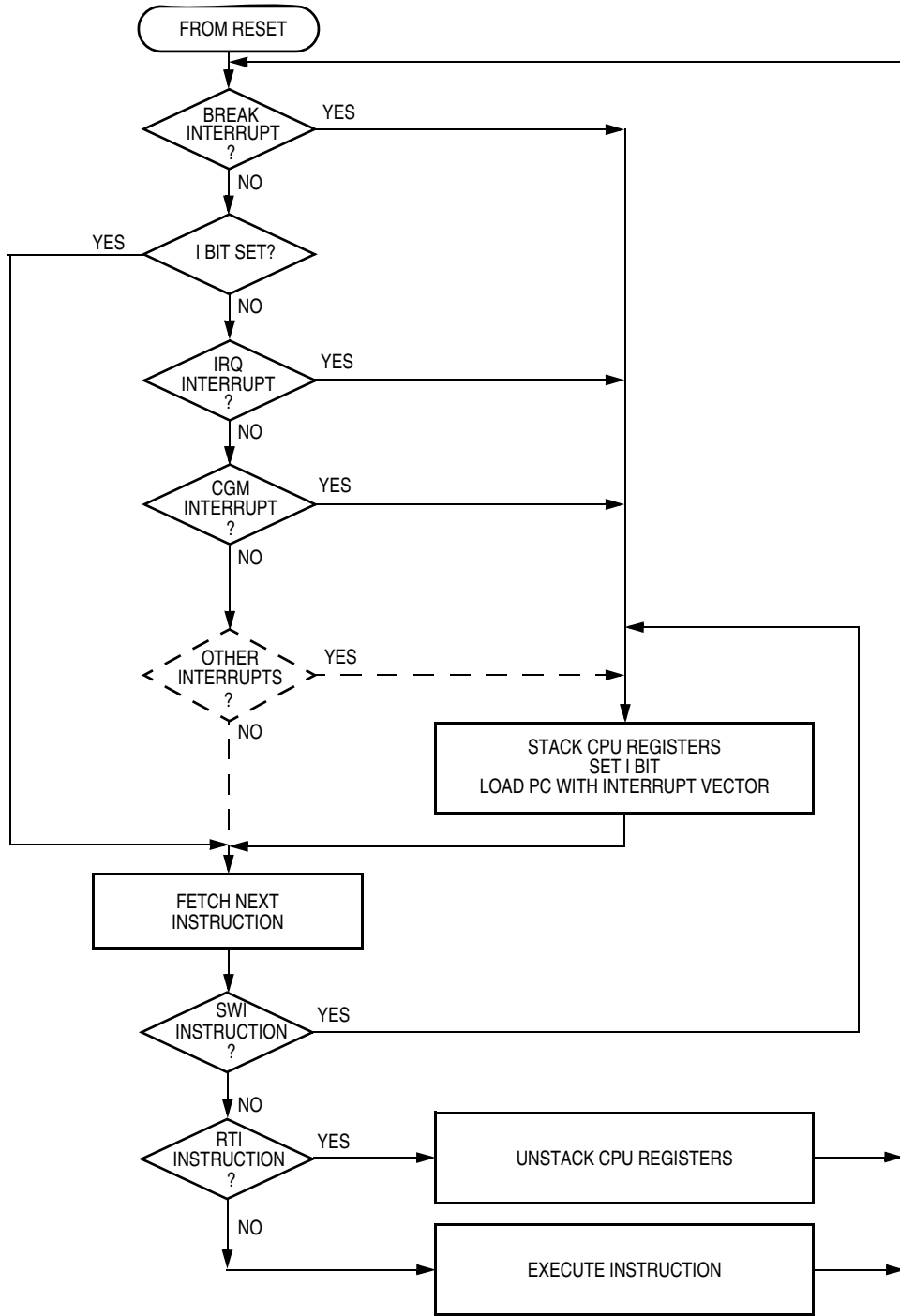
Figure 14-5. Interrupt Processing
