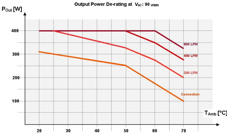
Figure 1. Power Derating Curves for Open Frame, U-Chassis and Perforated Cover Models
