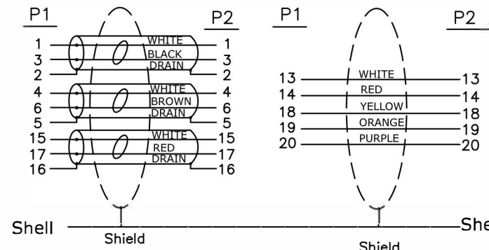
PIN Assignment
