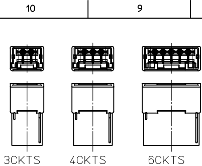
VIEW OF 3,4,6CKTS (SCALE 1:1)
