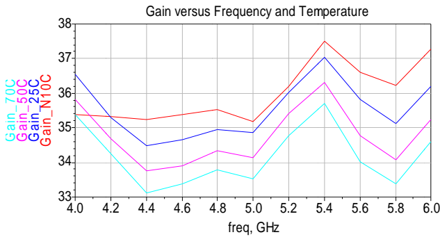
Figure 6 Gain vs Temperature
