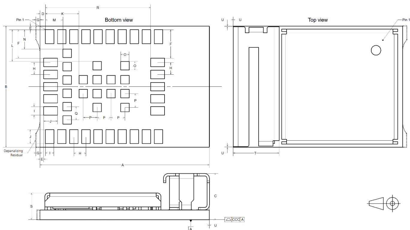
Figure 8: NINA-W132 mechanical outline
