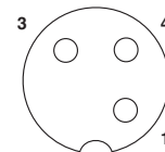
Pin assignment M12 socket, 3-pos.
