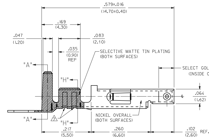
#18-24 TERMINAL SHOWN
