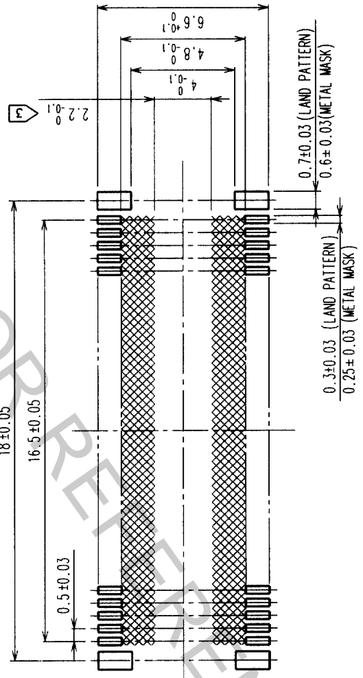
RECOMMENDED LAND PATTERN DIMENSION OF PCB
