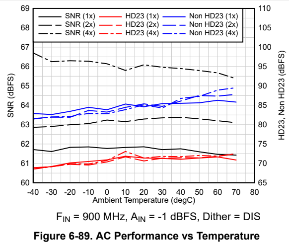
Figure 6-89. AC Performance vs Temperature
