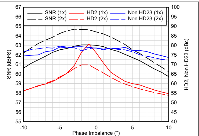
Figure 7-4. Phase Imbalance - 2.6 GSPS
