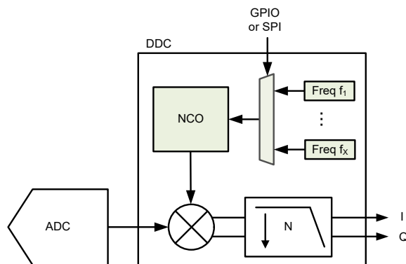
Figure 7-38. NCO Block Diagram
