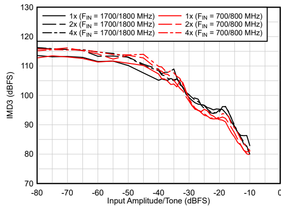
Figure 6-31. AC Performance vs A_{IN}
