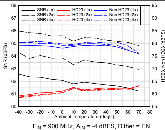
Figure 6-90. AC Performance vs Temperature
