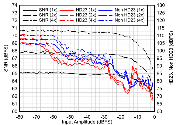
F_{IN} = 900 MHz, Dither = DIS
