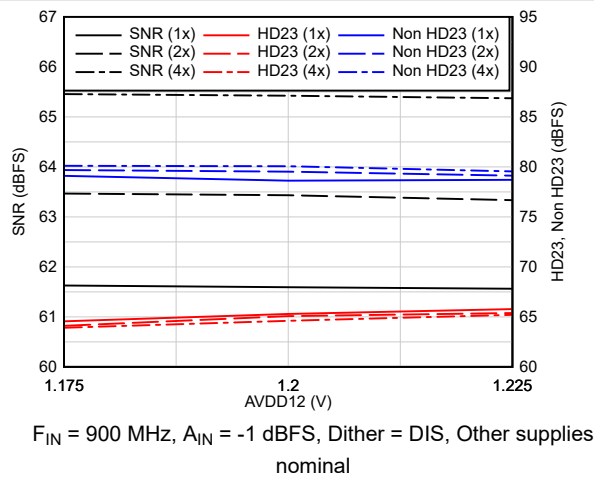
Figure 6-88. AC Performance vs AVDD12
