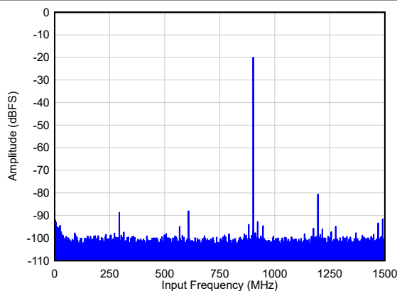
Figure 6-66. Single Tone FFT at F_{IN} = 900\text{ MHz}
