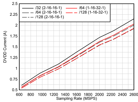
A_{IN} = -1 dBFS, 1x AVG, Dither = DIS Quad Band Decimation
