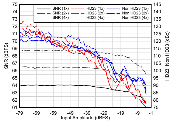
Figure 6-83. AC Performance vs A_{IN}
