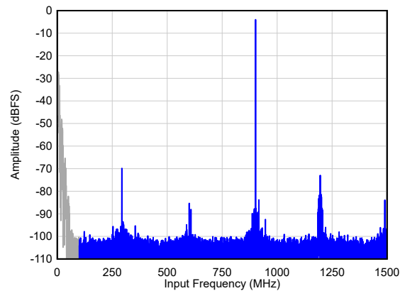
Figure 6-65. Single Tone FFT at F_{IN} = 900\text{ MHz}
