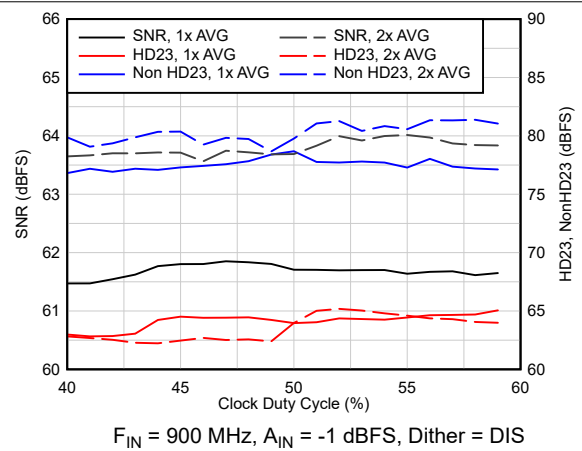
Figure 6-91. AC Performance vs Clock Duty Cycle
