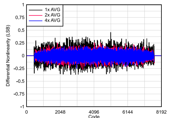
Figure 6-42. DNL vs Code
