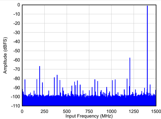
Figure 6-58. Single Tone FFT at F_{IN} = 1400\text{ MHz}
