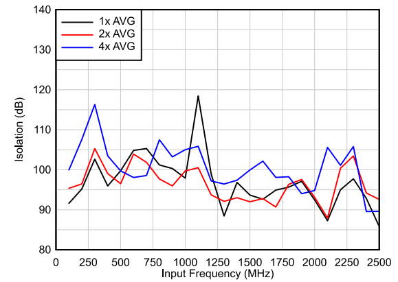
Figure 6-40. Isolation vs Input Frequency
