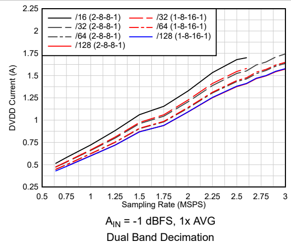
Figure 6-103. Current vs Sampling Rate vs Complex Decimation
