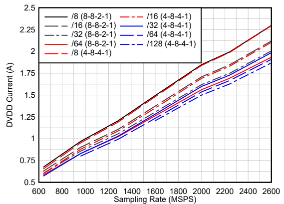
Figure 6-46. Current vs Sampling Rate vs Decimation
