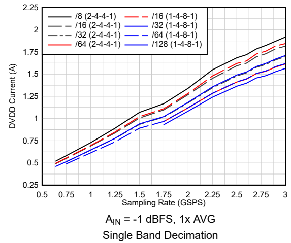
Figure 6-101. Current vs Sampling Rate vs Complex Decimation
