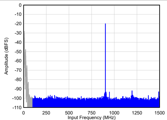
Figure 6-67. Single Tone FFT at F_{IN} = 900\text{ MHz}
