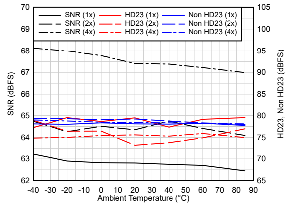
Figure 6-38. AC Performance vs Temperature
