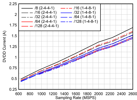
Figure 6-45. Current vs Sampling Rate vs Averaging
