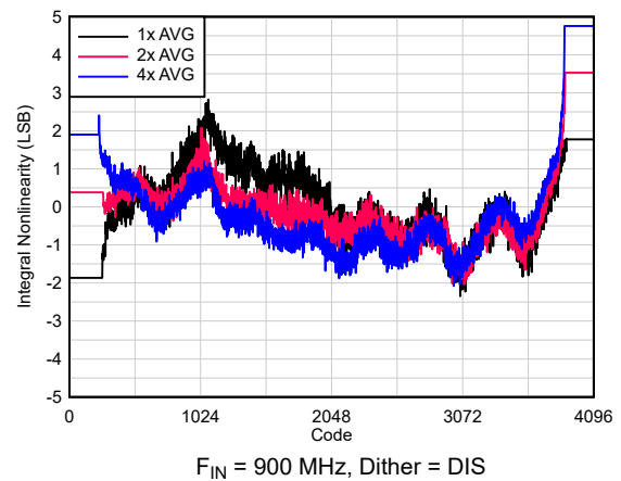
Figure 6-93. INL vs Code
