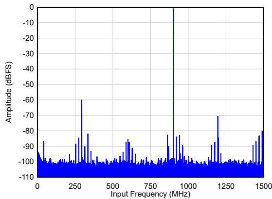
Figure 6-64. Single Tone FFT at F_{IN} = 900\text{ MHz}
