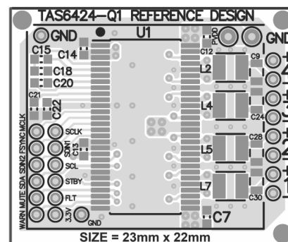
PCB AREA
