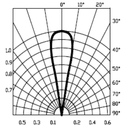
Radiation Diagram
