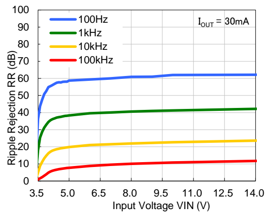
VR=3.3V, I_{OUT}=30\text{mA}
