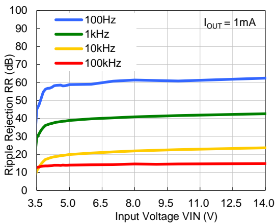
VR=3.3V, I_{OUT}=1\text{mA}
