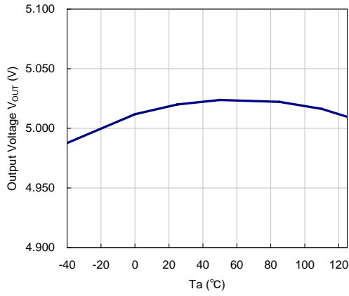
VR=5.0V
