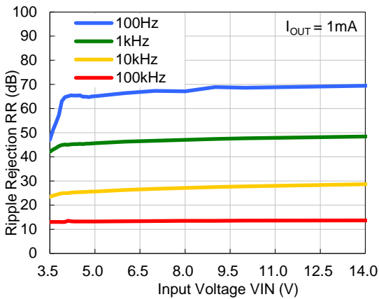
VR=3.3V, I_{OUT}=1\text{mA}
