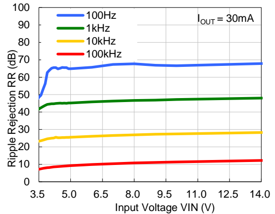
VR=3.3V, I_{OUT}=30\text{mA}
