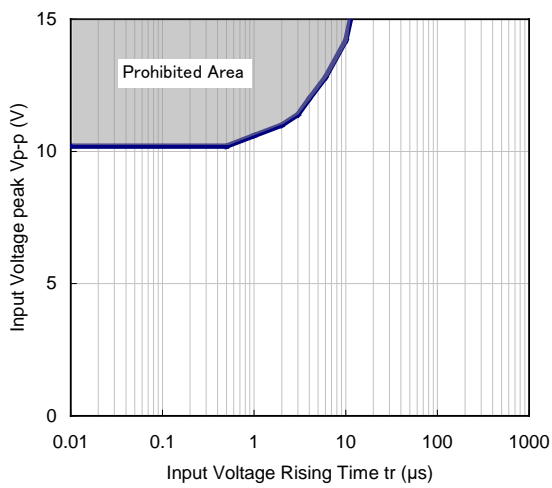
Prohibited Area of Fluctuation at Rising of V_{IN}
