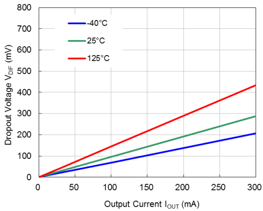
VR=5.0V
