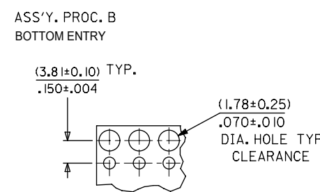
RECOMMENDED P.C. BOARD LAYOUT FOR ASS'Y. PROC. B
