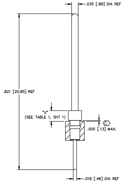
FIG. 22 TERMINAL STYLE -K T-1R12-X
