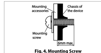
Fig. 4. Mounting Screw
