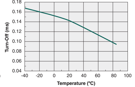
Typical Turn-Off Time vs. Temperature ( I_F=10\text{mA} , I_L=0.4A_{DC} )
