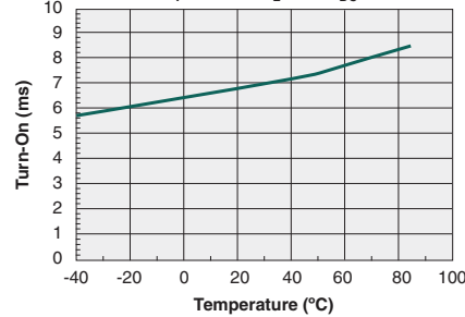
Typical Turn-On Time vs. Temperature ( I_F=10\text{mA} , I_L=0.4A_{DC} )
