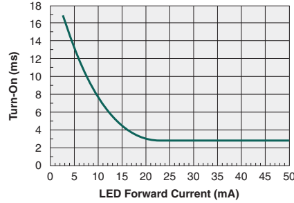
Typical Turn-On Time vs. LED Forward Current ( I_L=0.4A_{DC} )
