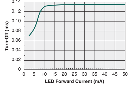
Typical Turn-Off Time vs. LED Forward Current ( I_L=0.4A_{DC} )
