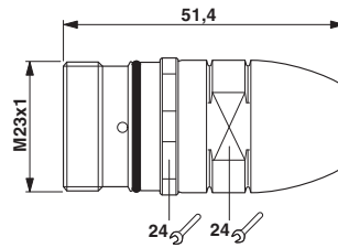
Dimensioned drawing
