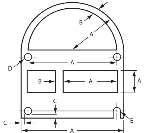
Figure 1 DIE-CUT GASKET
