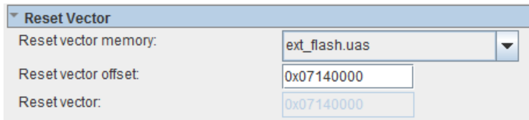
Figure 4-7 Factory Software Reset Vector Settings for NIOS II Processor
