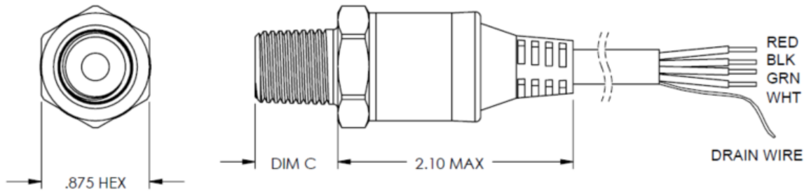
Digital Output Connection (Cable Type)
