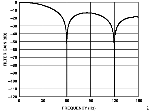
Figure 107. 60 Hz Rejection
