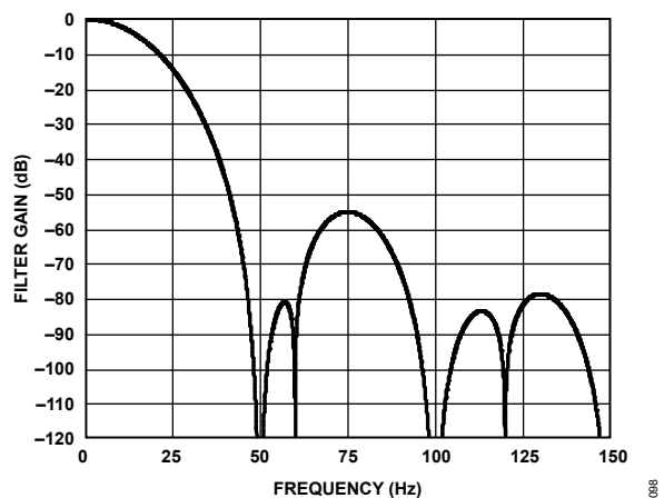
Figure 88. \text{Sinc}^4 Filter Response (50 SPS Output Data Rate, Zero Latency Disabled or 12.5 SPS Output Data Rate, Zero Latency Enabled, REJ60 = 1)
