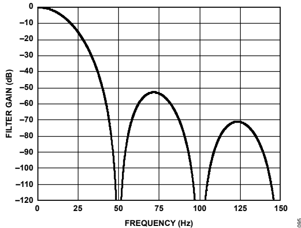
Figure 85. \text{Sinc}^4 Filter Response (50 SPS Output Data Rate, Zero Latency Disabled or 12.5 SPS Output Data Rate, Zero Latency Enabled)
