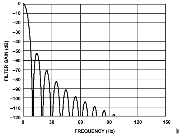
Figure 87. \text{Sinc}^4 Filter Response (10 SPS Output Data Rate, Zero Latency Disabled or 2.5 SPS Output Data Rate, Zero Latency Enabled)
