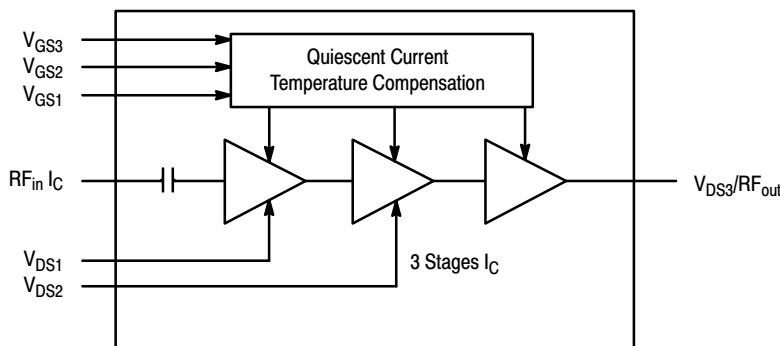
Figure 1. Block Diagram
