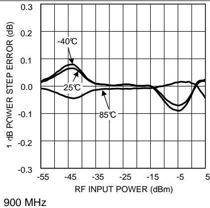
Figure 32. Error For 1-dB Input Power Step vs RF Input Power
