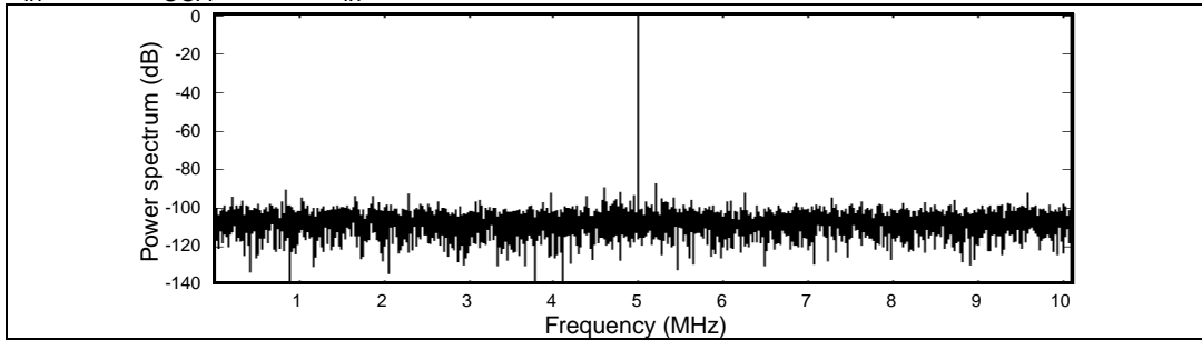
Figure 22. Dual-tone 8K FFT at 20Mpsps - Channel I
