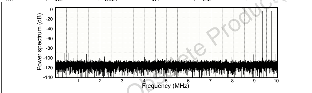
Figure 22. Dual-tone 8K FFT at 20Mpsps - Channel I
