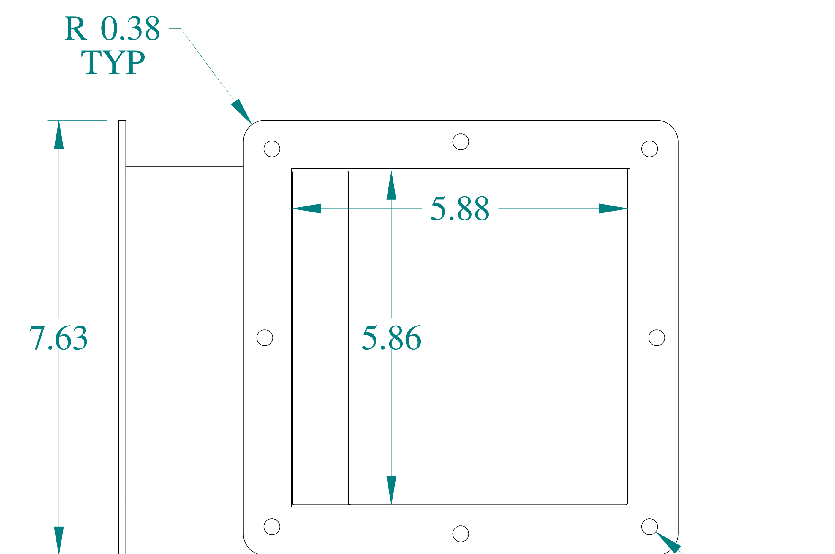
VIEW Z-Z
