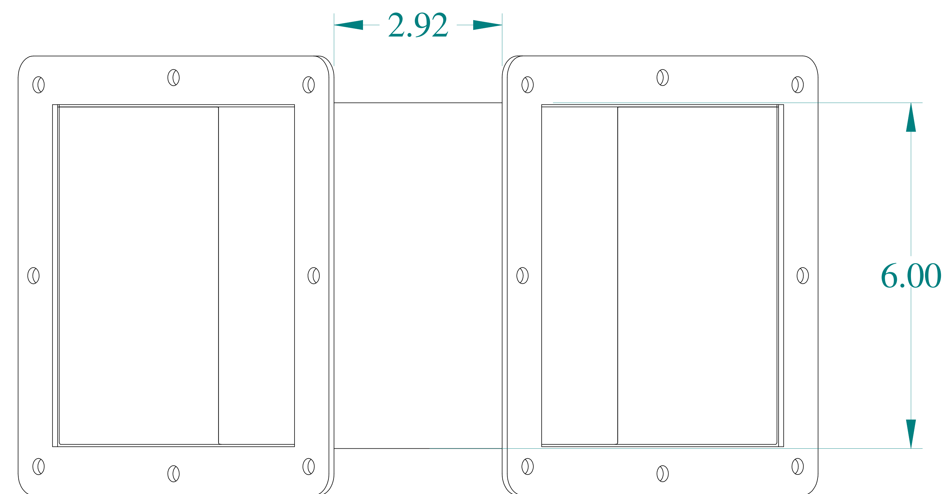
FRONT VIEW
