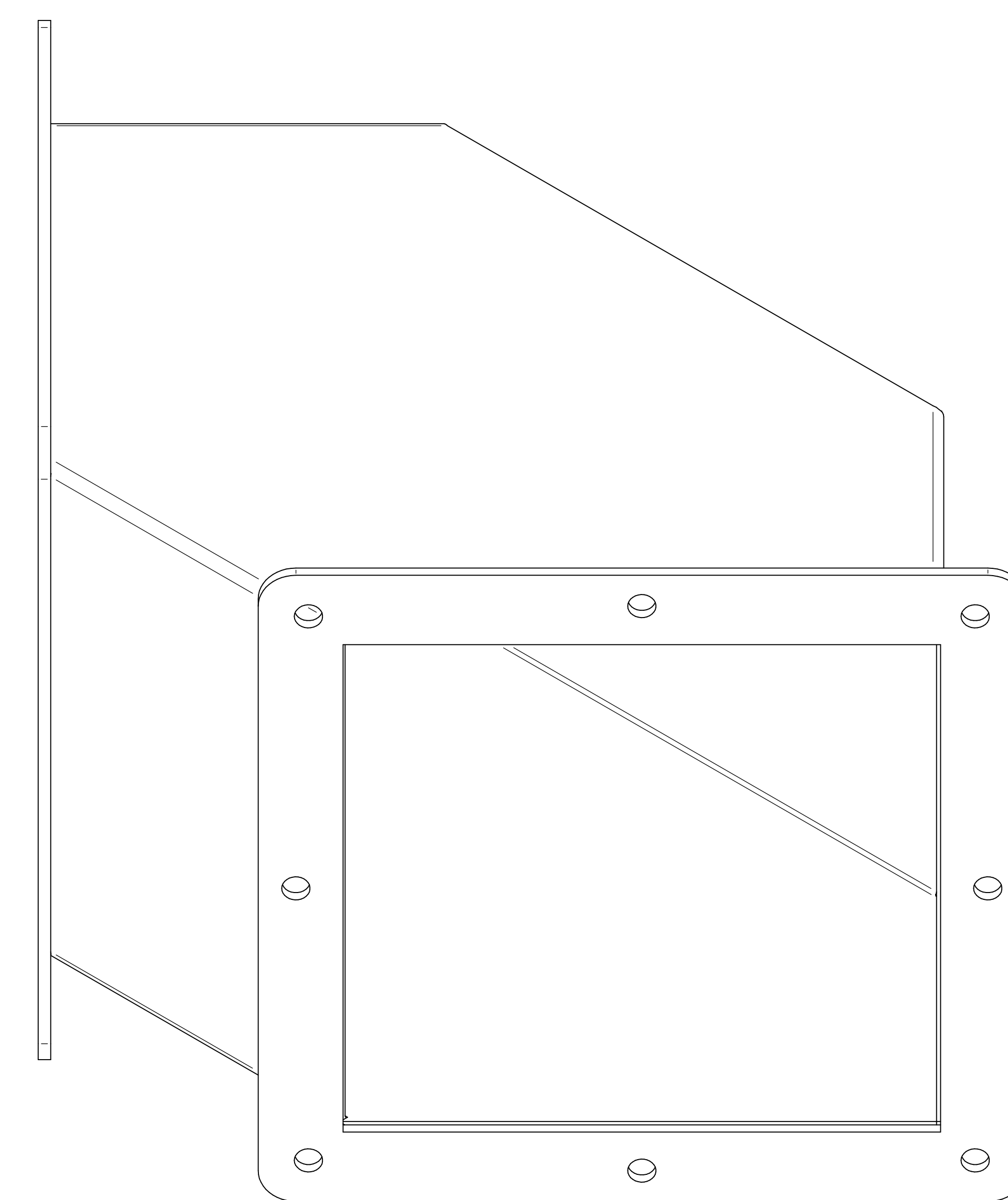
ISOMETRIC VIEWS
