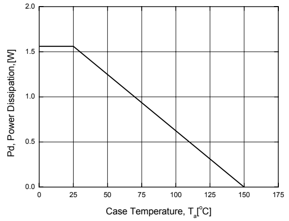
Figure 10. Power Derating
